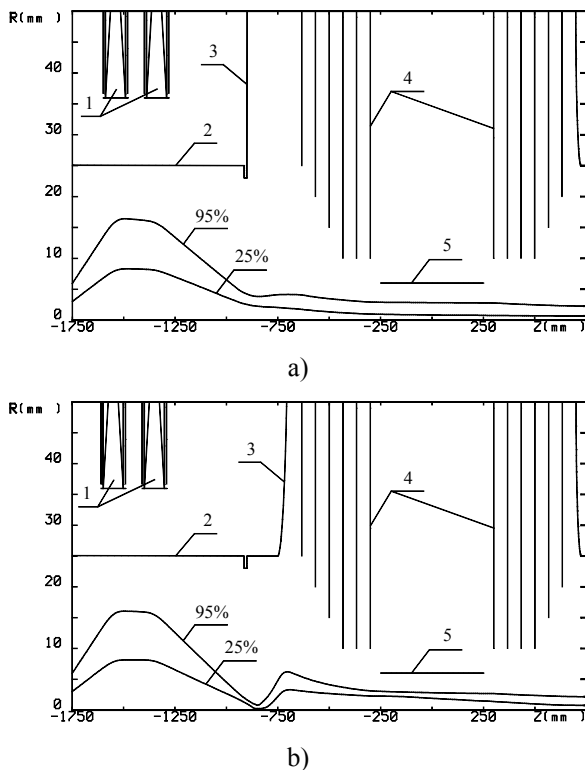
Figure 2: Computer simulated envelopes for "soft" (a) and "hard" (b) introduction of 10 mA beam into tandem accelerator. 1 – magnetic lenses, 2 – drift tube, 3 – vacuum tank, 4 – high-voltage electrode, 5 – charge-exchange tube
