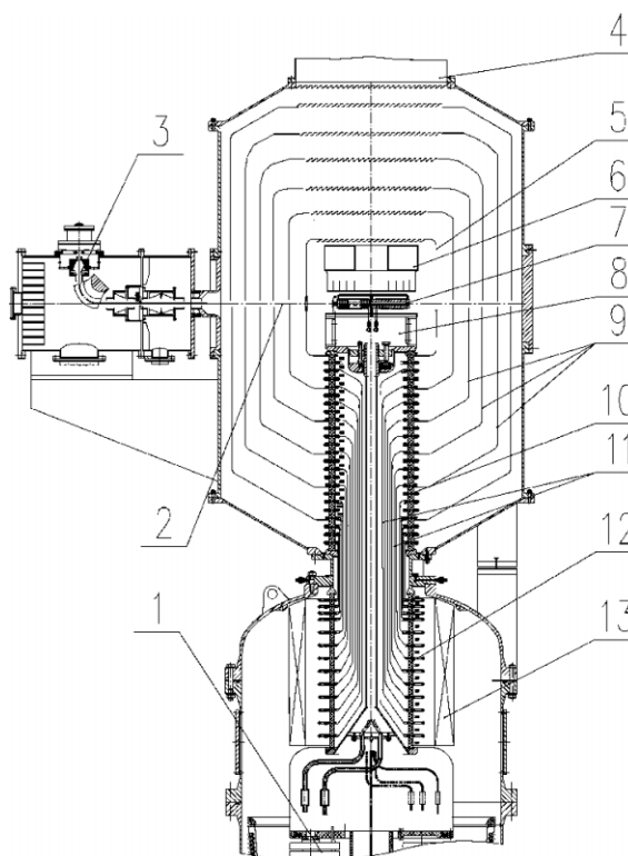
Figure 1: Vacuum insulation tandem
