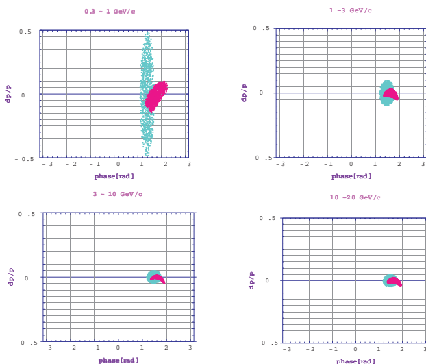
Fig. 2 Longitudinal particle simulations for FFAG chains.
