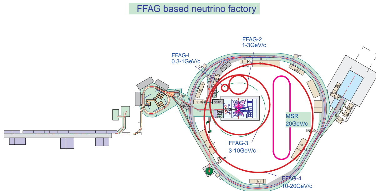
Fig.1 Conceptual schematic layout of the FFAG based neutrino factory with the 50 GeV proton driver at JAERI Tokai site.
