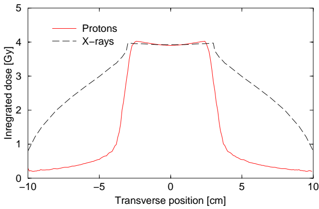
Figure 3: Integrated dose from tomotherapy of a 6 cm tumor using protons and X-rays. The collateral dose with protons is an order magnitude less than with X-rays.
