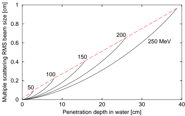
Figure 4: Transverse beam size due to multiple scattering.
