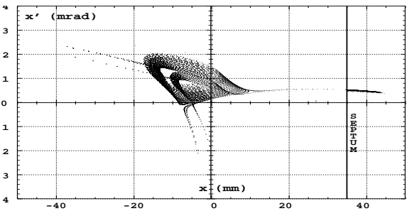
Figure 5: Horizontal phase space at extraction.
