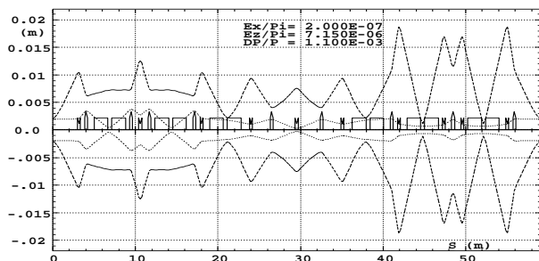
Figure 7: Typical envelopes in the 59 m long vertical beam line.
