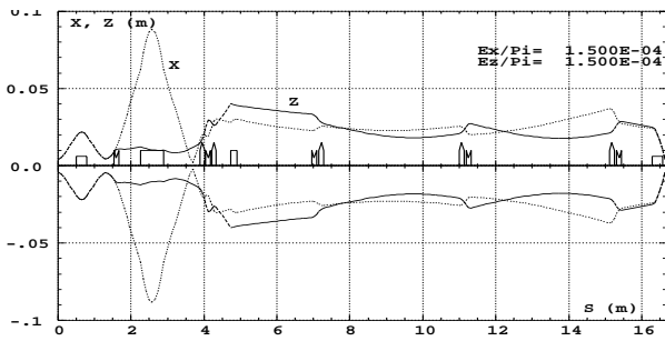
Figure 2: Beam envelopes in the LEBL (no space charge).
