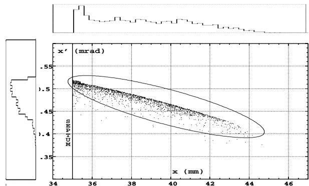
Figure 6: Extracted beam at entrance to the electrostatic septum.
