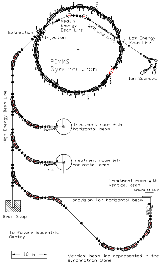
Figure 1: General structure of the facility
