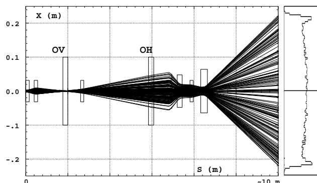
Figure 8: Uniformized cross-section at target, by octupole lenses OH and OV.
