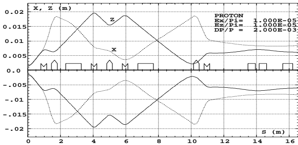
Figure 3: Beam envelopes in the MEBL (proton case).
