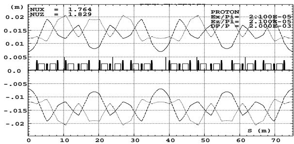
Figure 4: 7 MeV p-beam stored envelopes after injection.
