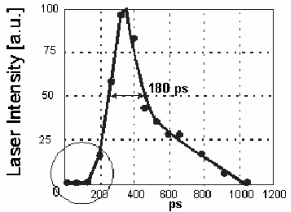
Figure 1: Measured time profile of the CO 2 beam after the preamplifier
