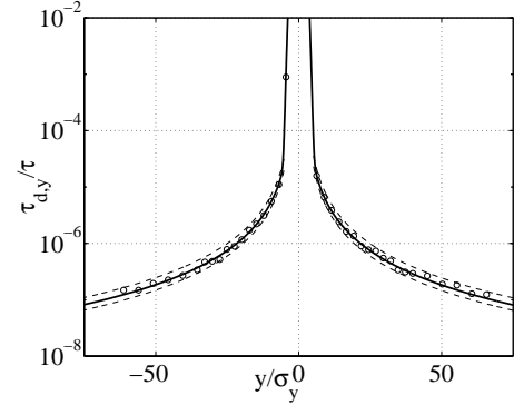
Figure 1: Inverse beam lifetime normalized on the inverse vertical damping time versus position of the vertical top and bottom scrapers normalized on the vertical beam size. Dots show the experimental data and solid line shows the fit. The dashed lines show the error margins for a 1\sigma confidence level.
