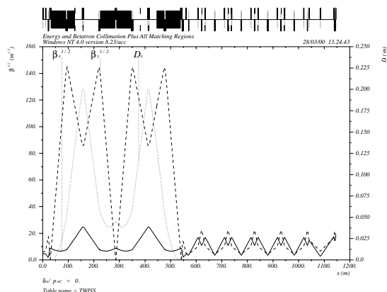
Figure 2: Optical functions of proposed new NLC post-linac collimation system.
