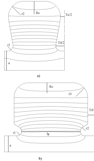
Figure 1: Geometry definition for different shapes of the DLW (a) and CCS (b) cells.
