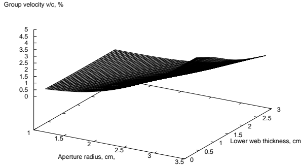
Figure 2: The surface \beta_g(a, T_d) for a DLW with r_1 = 0.3\text{cm} , T_u = 1.2\text{cm}
