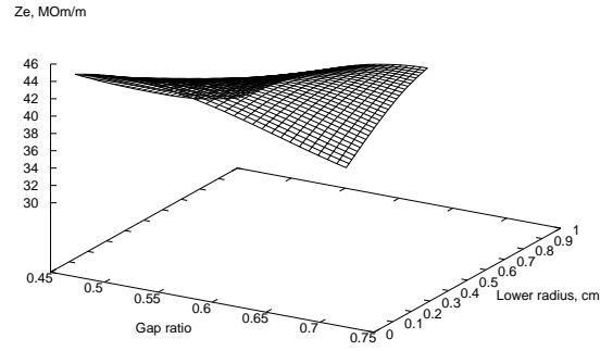
Figure 3: The surface of Z_e(\alpha_{gp}, r_1) for a SW structure cell with a = 2.0\text{cm} , T_d = 3.0\text{cm} .
