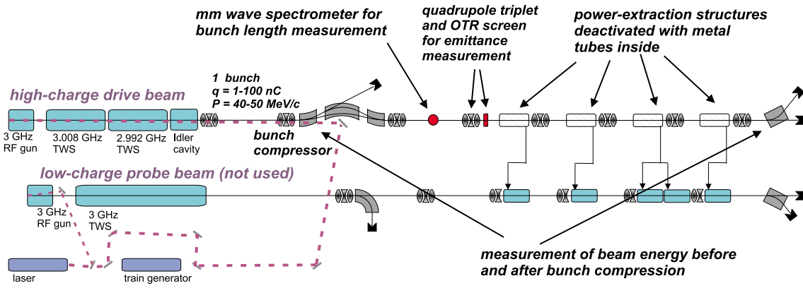
Figure 1: The second CLIC Test Facility CTF II. The CSR experiments were performed on the drive beam (upper part).
