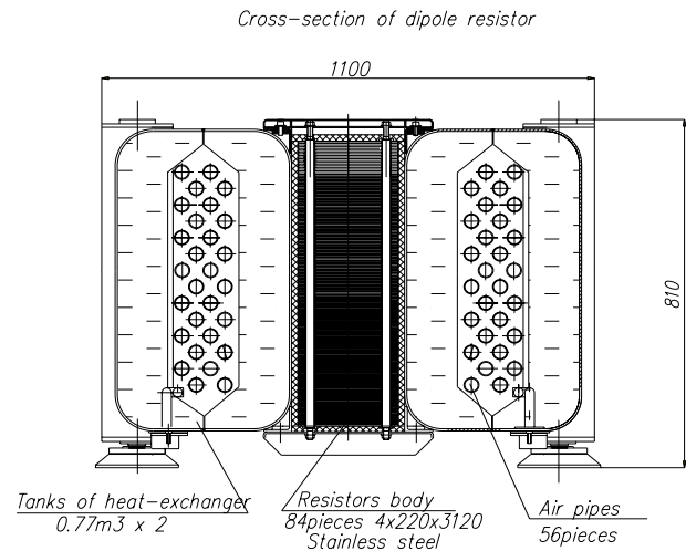
Fig. 1. Cross sections of a 225 mΩ and 3.5 m long dipole resistor
