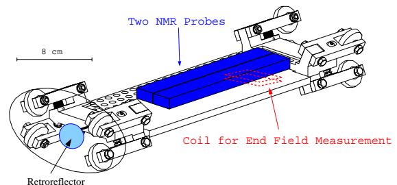
Figure 2: Schematic diagram of the mole.
