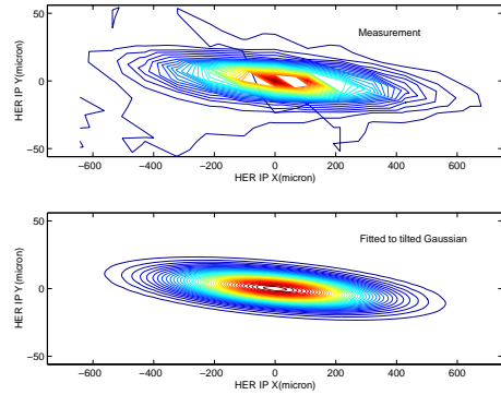
Figure 3: Two dimensional luminosity scan for PEP-II
