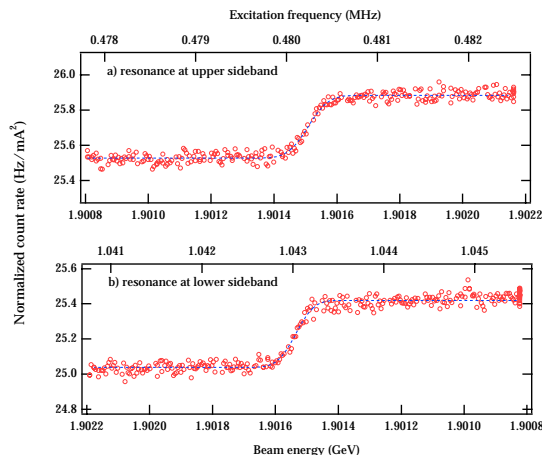
Figure 2: Normalized loss detector rate during excitation sweep of spin resonances. a) Sweep through upper sideband and b) lower sideband.
