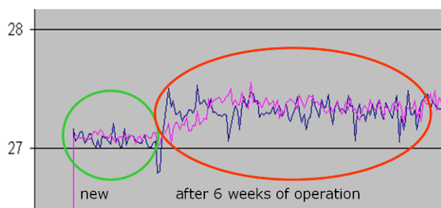
Figure 3: Representative “empty” signal from the first CCD camera, i.e. average over non-illuminated sector of frame, at the start (green circle) and at the end (red oval) of the VIMOS service period. Due to hot pixels the background level shifted just noticeable after irradiation, and fluctuations from frame to frame increased.
