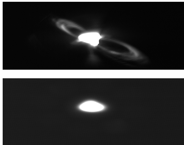
Figure 1: Set-up of the VIMOS camera by means of a special tool with a light emitting diode five years apart. Whereas the top image from the very start of operation features some reflections, nothing of this kind is visible after “seasoning” of the mesh. The absence of reflected light is consistent with the observed decrease in overall signal during the first year of irradiation.
