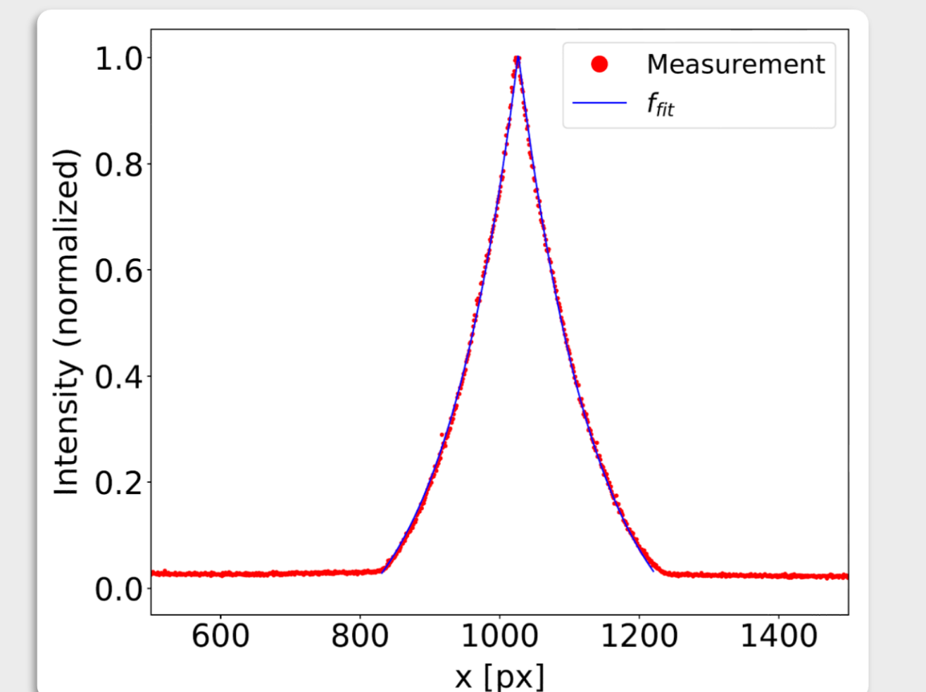
Fig.9: BIF profile with a 550 mA electron beam and the derived fit function
