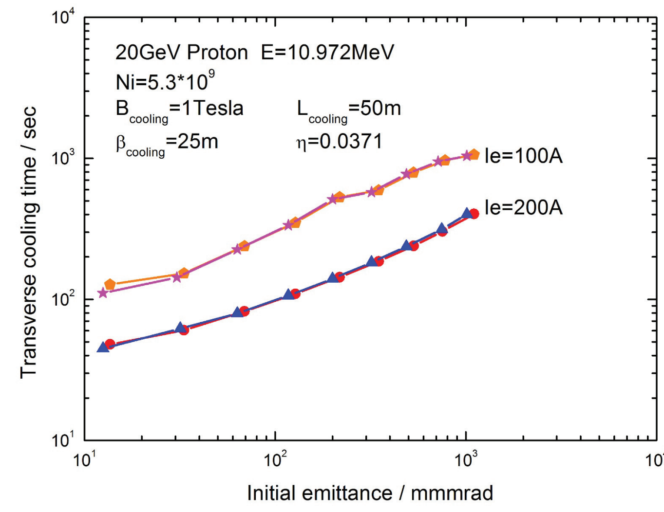
Figure 1: The transverse cooling time as a function of the initial emittance under the different electron beam current .
