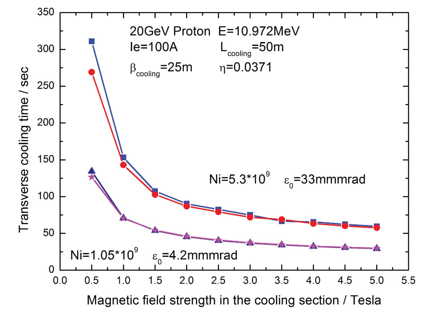
Figure 6: The transverse cooling time as a function of the magnetic field strength in the cooling section.
