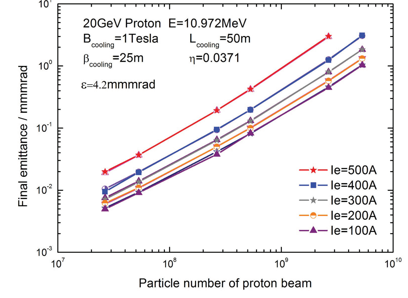
Figure 15: The final emittance as a function of the particle number in the proton beam.
