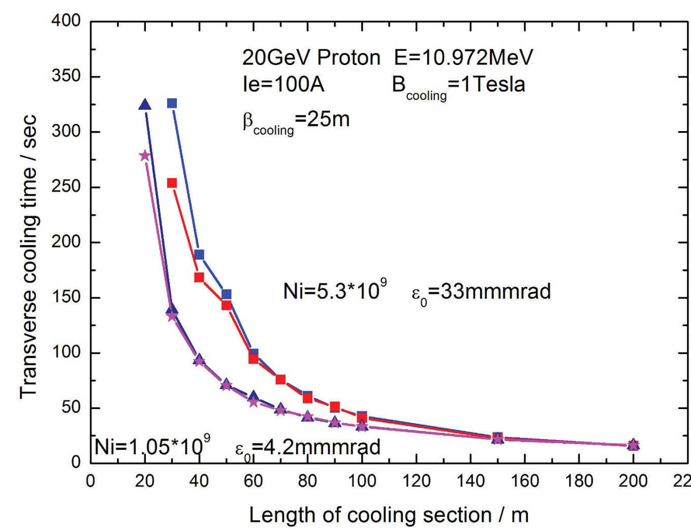
Figure 5: The transverse cooling time as a function of the length of the cooling section.
