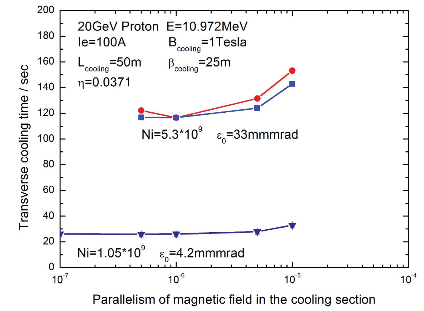
Figure 3: The transverse cooling time as a function of the parallelism of magnetic field in the cooling section
