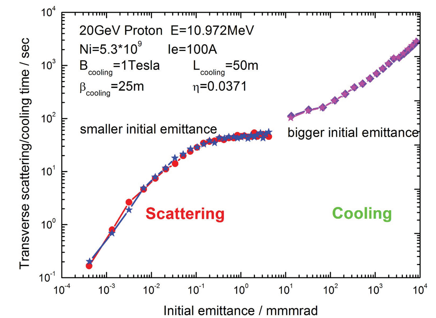
Figure 15: The transverse cooling /scattering time as a function of the initial emittance under 100A electron beam cooling.
