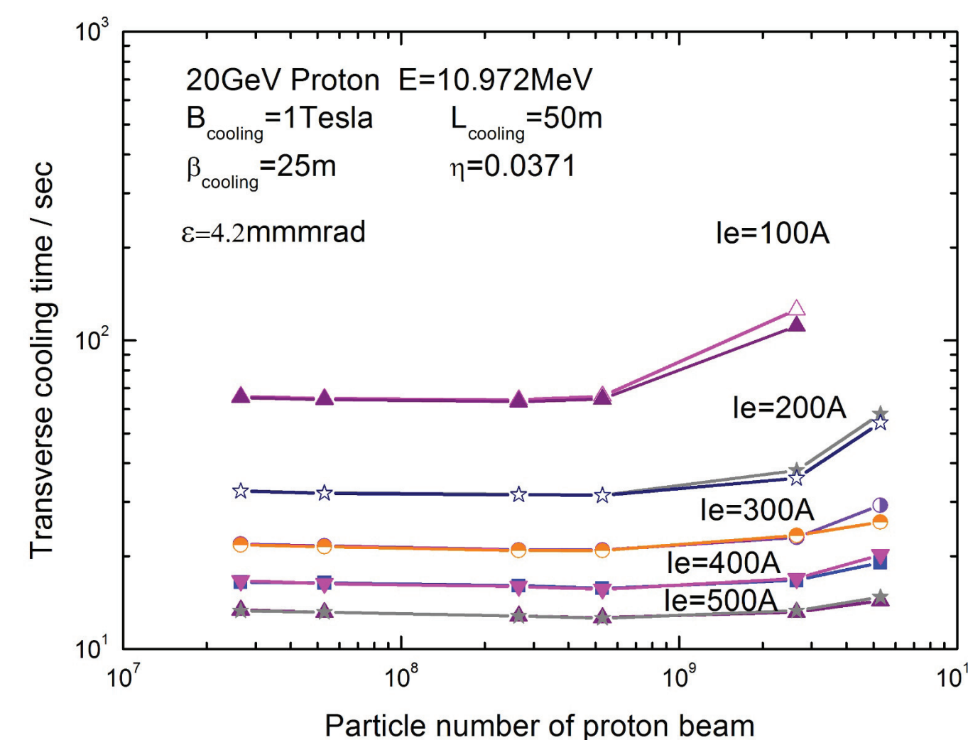
Figure 10: The transverse cooling time as a function of the particle number in the proton beam.
