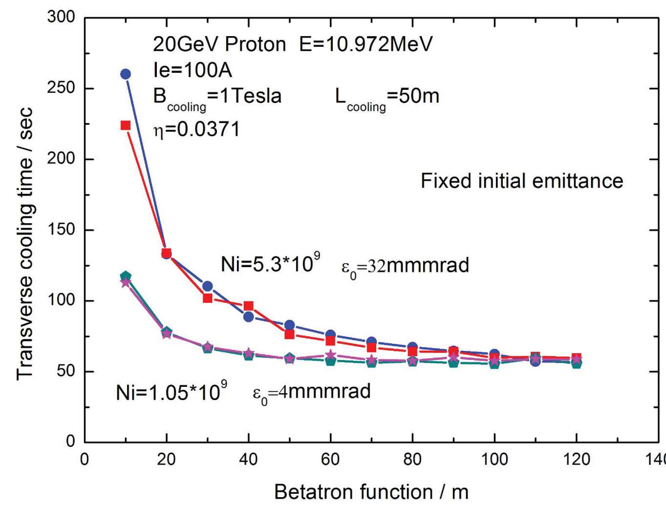
Figure 7: The transverse cooling time as a function of the Betatron function in the cooling section.
