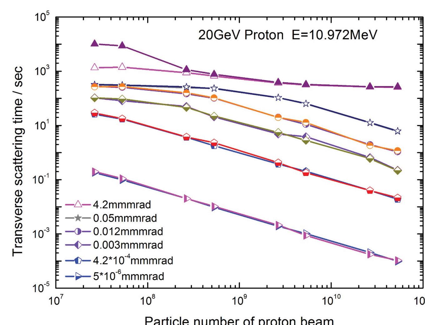
Figure 11: The transverse scattering time as a function of the particle number in the proton beam.
