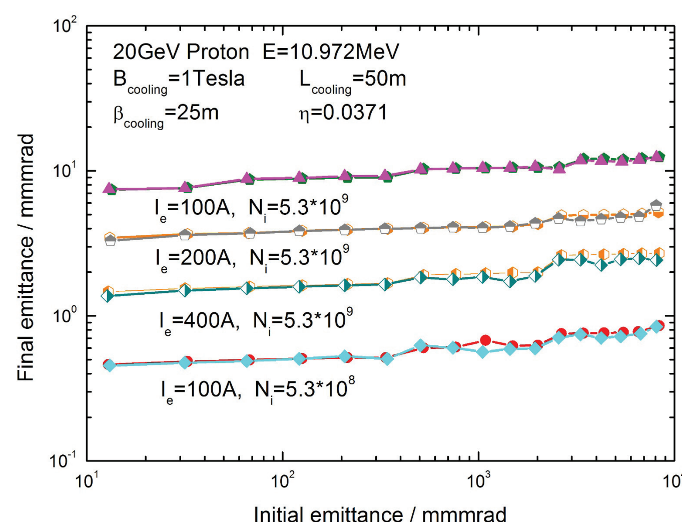
Figure 13: The final emittance as a function of the initial emittance of the proton beam in the case of different electron beam current.
