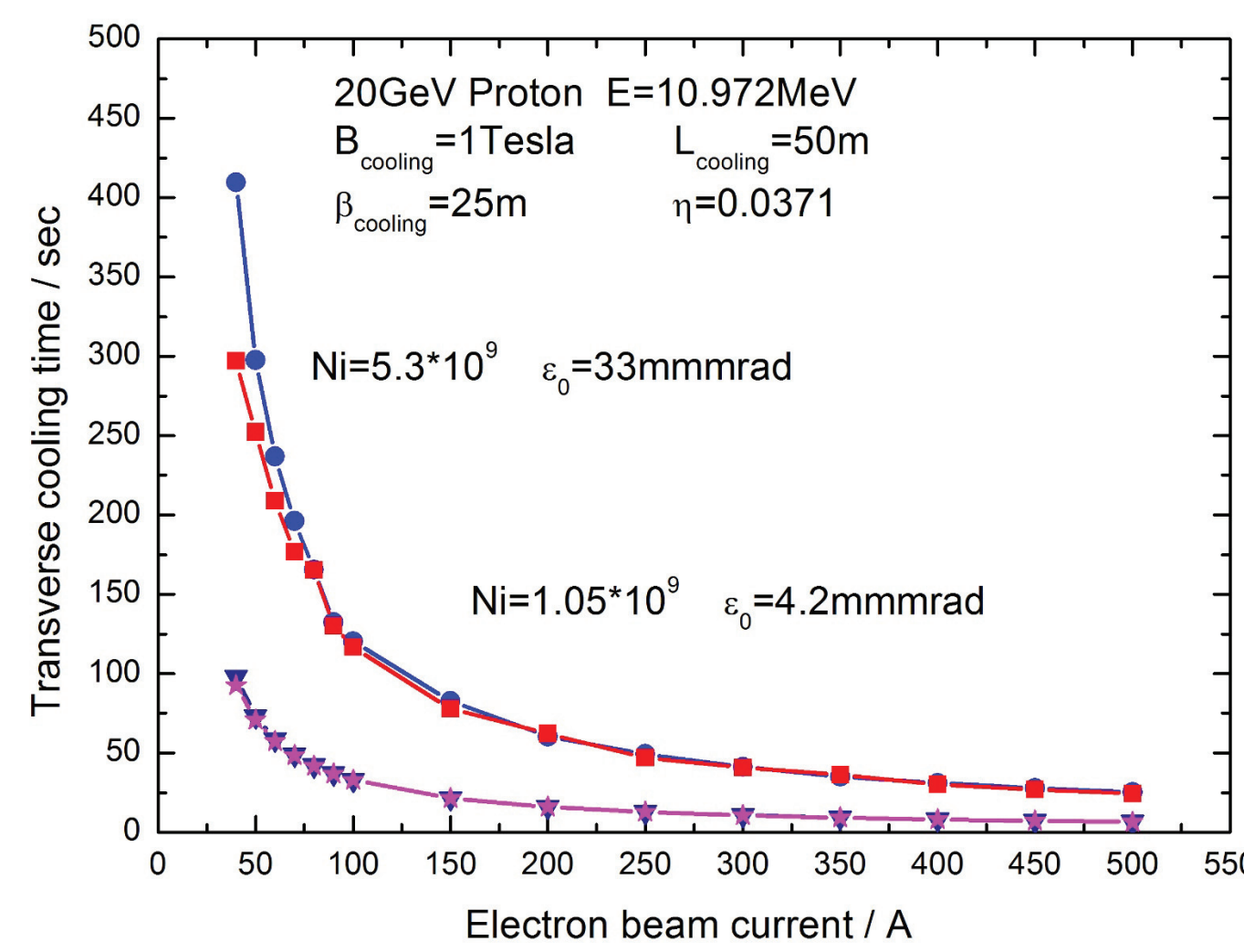
Figure 4: The transverse cooling time as a function of the electron beam current.
