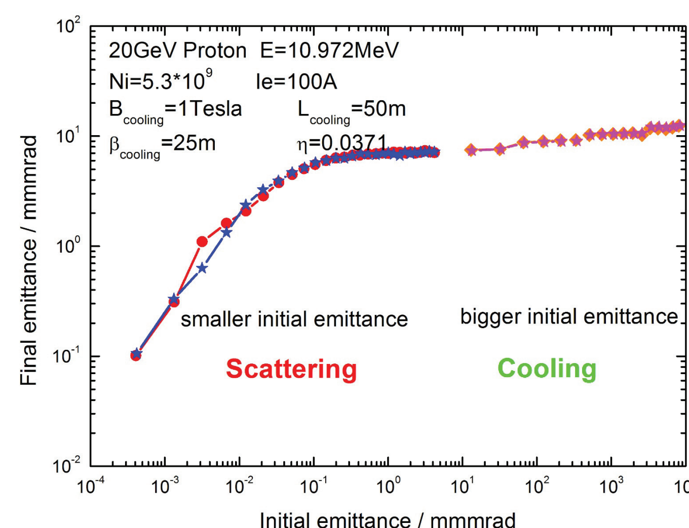
Figure 14: The final equilibrium emittance as a function of the initial emittance under 100A electron beam cooling.
