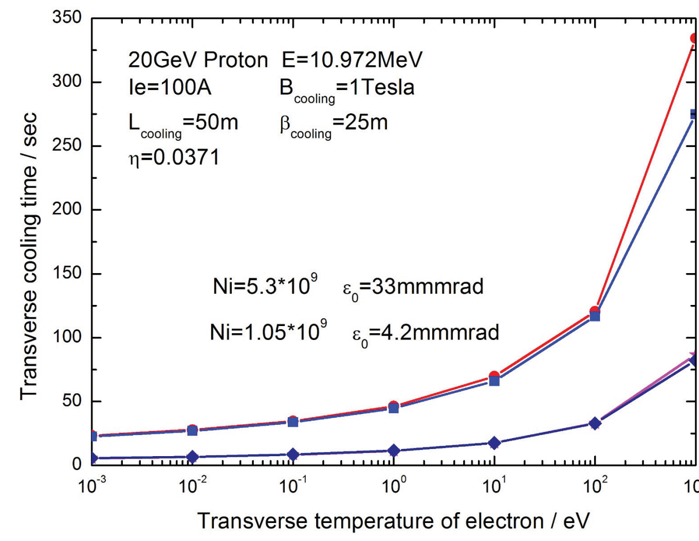
Figure 2: The transverse cooling time as a function of the transverse temperature of electron beam in the cases of different proton number.
