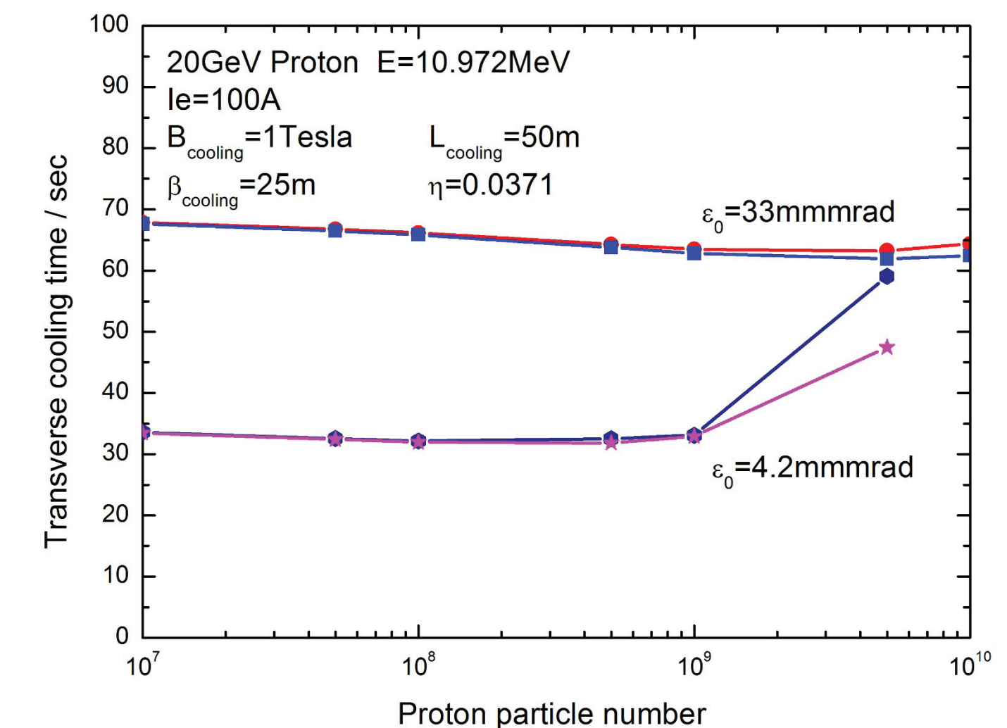
Figure 9: The transverse cooling time as a function of the particle number in the proton beam.
