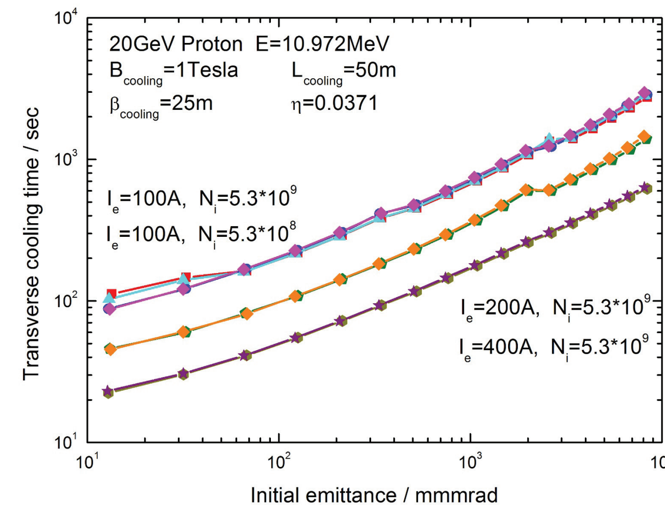
Figure 8: The transverse cooling time as a function of the initial emittance under the different electron beam current.
