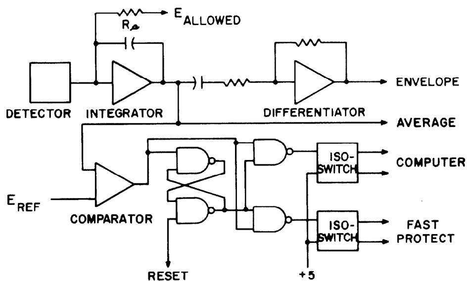
SIMPLIFIED SYSTEM DIAGRAM
