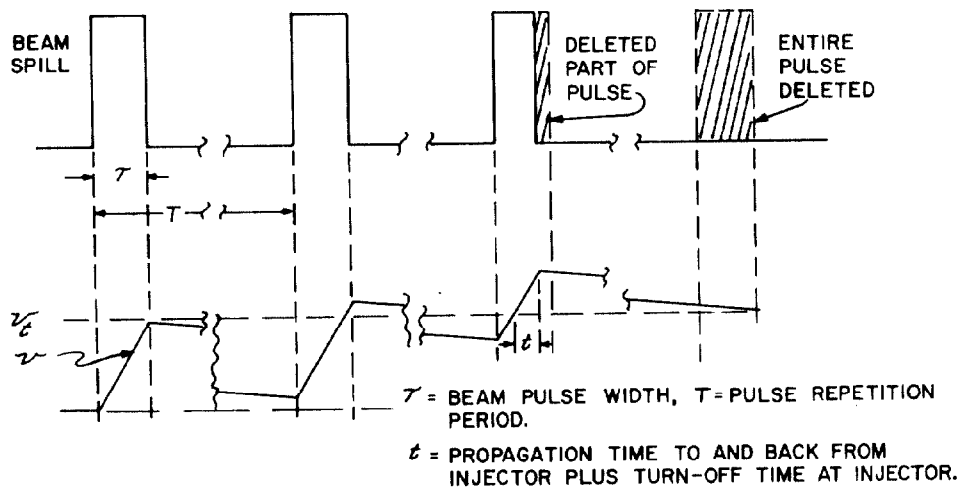
BEAM PULSE MODULATION BY BEAM SPILL CONTROL SYSTEM
