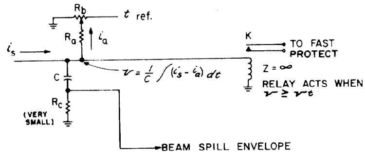
CONCEPTUAL BEAM SPILL CONTROL SYSTEM
