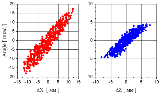
Figure 5 The horizontal and vertical emittances of the extracted beam ( A/Z=8 , B_0=1.45 T)
