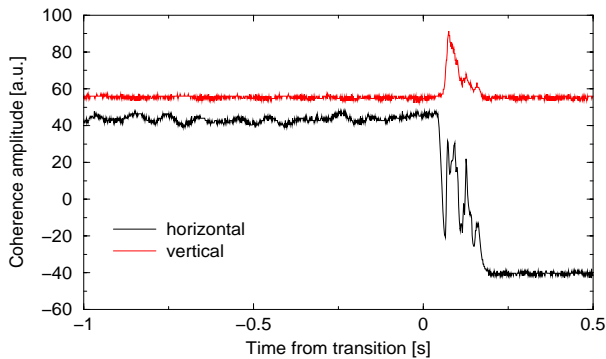
Figure 9: Coherence signal of bunch #40 from the turn-by-turn BPM data. The horizontal instability signal is within a step caused by the orbit shift due to \gamma_T -jump.
