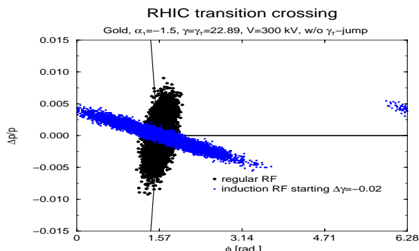
Figure 15: Longitudinal phase space showing the reduction of peak bunch density near \gamma_T using an induction RF system [24].
