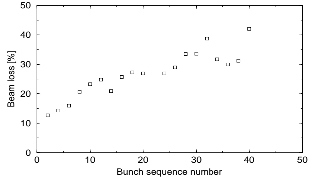
Figure 6: Beam loss at transition as a function of bunch sequence number with V_{rf} = 200 kV and b_{oct} = -3 unit. Major machine parameters are listed in Table 1.
