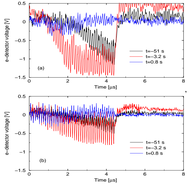
Figure 5: Electron flux measured in the (a) horizontal and (b) vertical directions near transition ( \gamma_T ) at t = 0 . An ac-coupled amplifier is used with a low-frequency cut-off of about 300 kHz. The grid is not biased. The collector is biased at 50 - 100 V positive.
