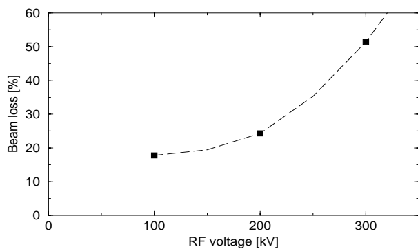
Figure 14: Average beam loss at \gamma_T as a function of the RF voltage with b_{oct} = -3 unit.
