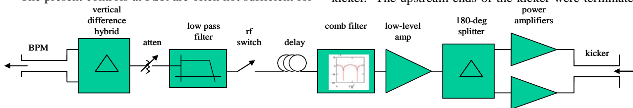
Figure 1. Block diagram of the prototype damping system tested at PSR. Beam direction is right to left.
