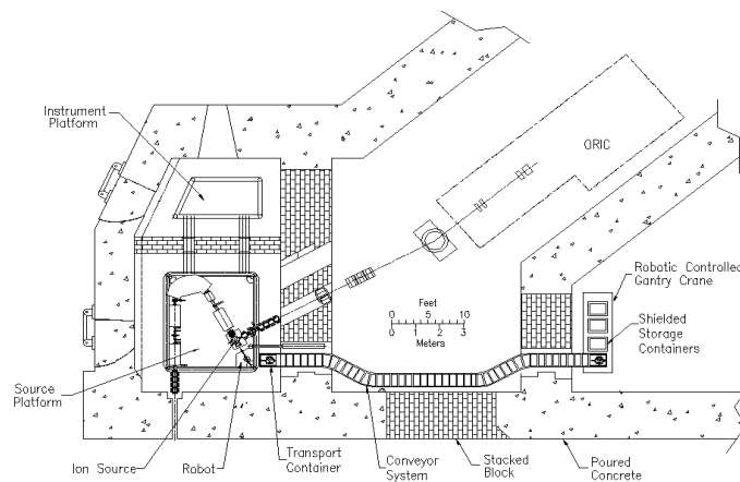
Fig. 3. Schematic representation of the RIB injector for the 25-MV tandem accelerator and the radiation handling system for installation/removal/storage/disposal of radioactively contaminated targets and ion sources.
