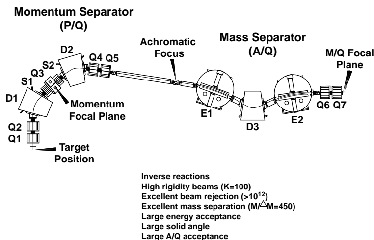
Fig. 6. Schematic drawing of the Recoil Mass Spectrometer (RMS) showing the principal components used to separate recoils from the primary ion beams.
