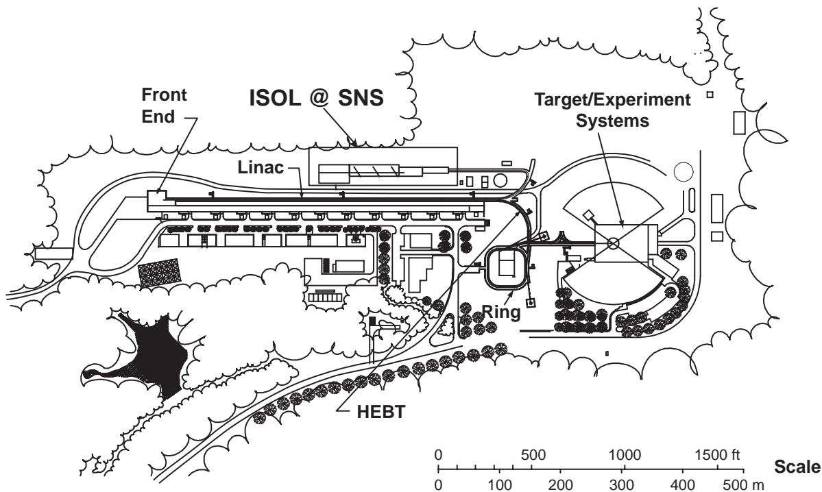
Fig. 8. Preferred scenario for a second generation ISOL facility located in close proximity to the Spallation Neutron Source (SNS) facility. The ISOL facility would rely on pulsed manipulation of a 1-GeV 1\text{-}\mu\text{A} \text{H}^- ion beam to divert 100 \mu\text{A} for production of radioactive species.
