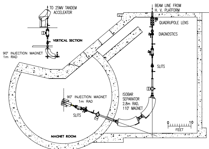
Fig. 4. Schematic representation of the injection line between the high voltage injector and 25-MV tandem electrostatic accelerator showing the magnetic isobar separation system.
