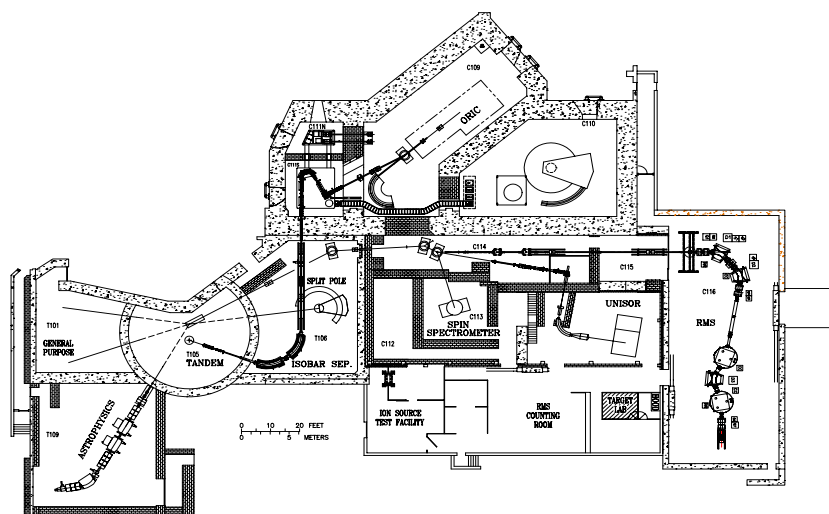
Fig. 1. Schematic layout of the Holifield Radioactive Ion Beam Facility (HRIBF) showing the principal components of the facility.
