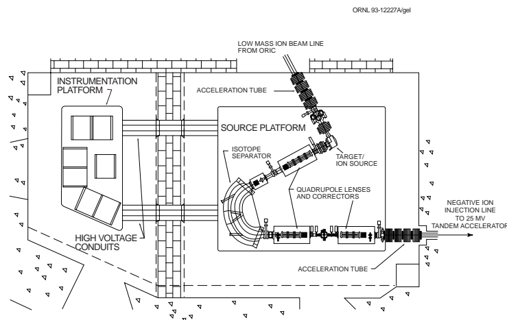
Fig. 2. Schematic drawing of the high voltage injector for the HRIBF 25-MV tandem electrostatic accelerator.
