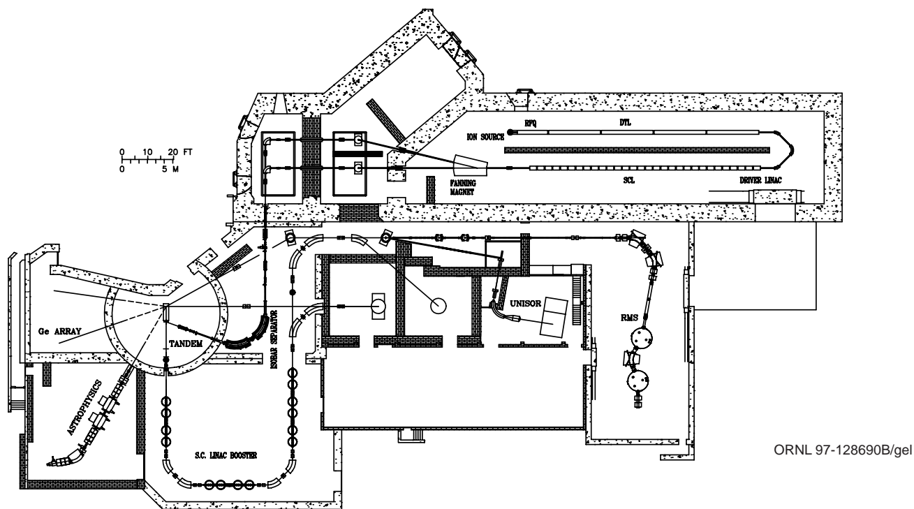
Fig. 7. Proposed scenario for a second generation HRIBF with a linear accelerator with capabilities of accelerating particles with Q/A = 1/2 up to 50 MeV and Q/A = 1 up to 200 MeV with respective intensities of 200 \cdot A on target. The targets are assumed to be vertically oriented.
