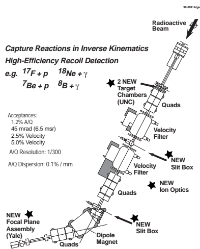
Fig. 5. Schematic drawing of the Daresbury Recoil Separator (DRS) as modified for nuclear astrophysics research at the HRIBF
