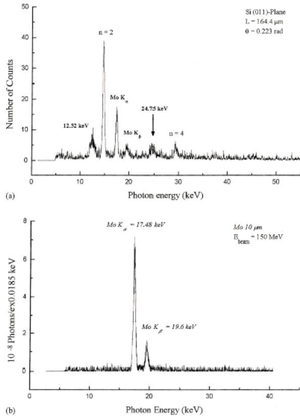
Figure 2: (a) PXR from (011) plane in 164.4 \mu\text{m} silicon crystal with the amorphous Mo target. (b) Spectrum from the amorphous Mo target [8].
