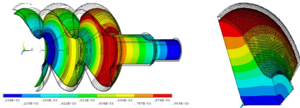
Figure 4: Elliptic cavity deformations by cool-down
