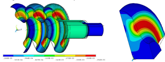
Figure 5: Elliptic cavity deformations under 1 bar wall pressure
