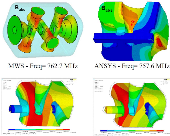
Figure 12: Triple-spoke cavity cool-down simulations
