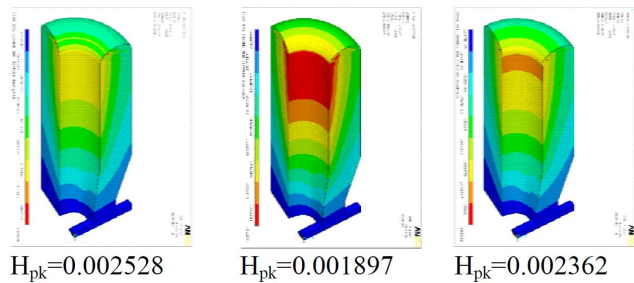
Figure 7: HWR magnetic field distribution with different mesh around B_{pk} region
