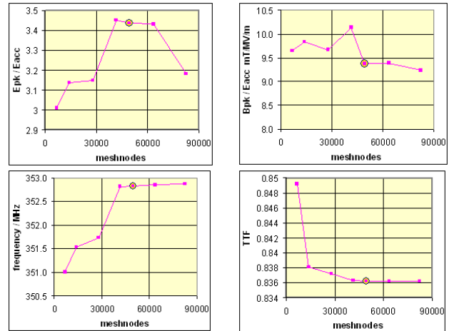
Figure 10: Cavity parameter dependences on mesh dense.
