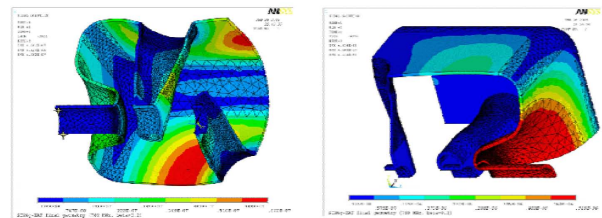
Figure 14: Triple-spoke cavity LFD simulations
