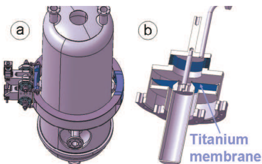
Figure 7: \beta=0.12 tuners
