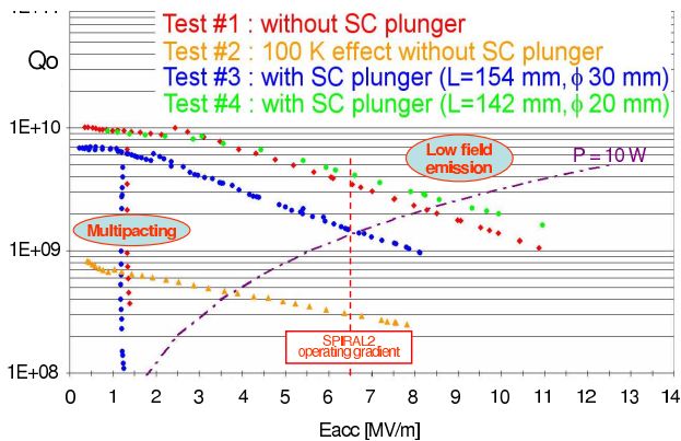
Figure 9: \beta=0.12 prototype cavity 4 K tests
