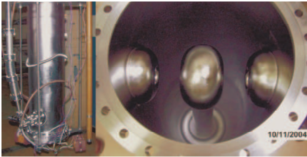
Figure 4: \beta=0.07 prototype cavity
