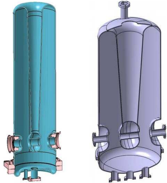
Figure 1: \beta=0.07 (left) and \beta=0.12 (right) QWRs
