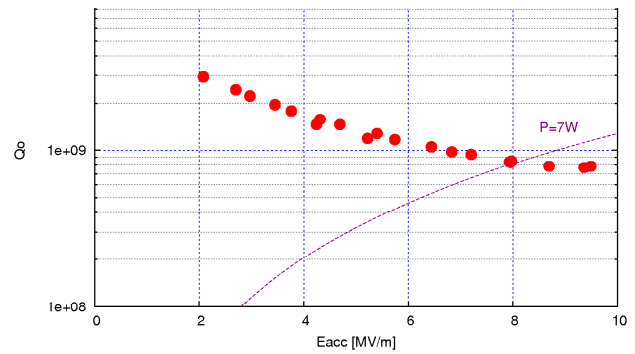
Figure 5: \beta=0.07 prototype cavity 4 K test
