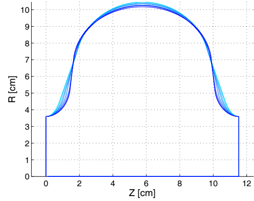
Figure 5: Plot comparing the geometry of the selected center cell shapes. Note that despite the significant geometry variation among them, though they all possess very similar fundamental mode properties.
