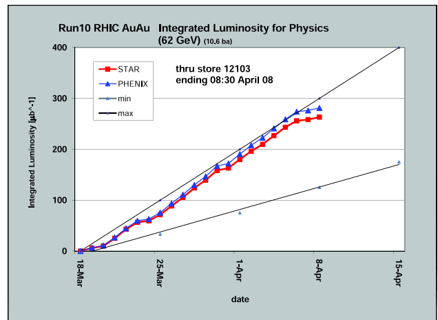
Figure 5: Integrated luminosity for RHIC operation at 31.2 GeV.
