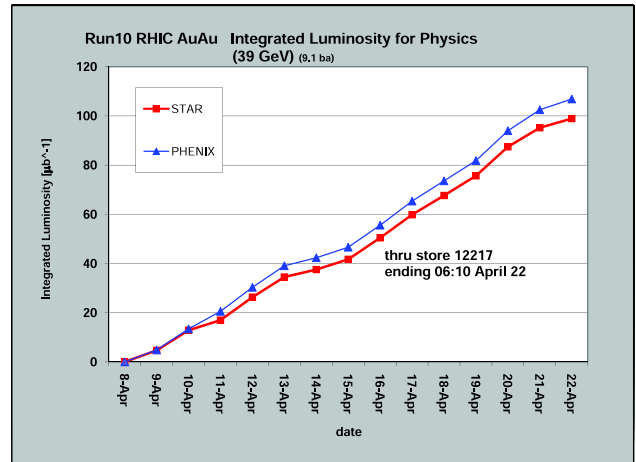
Figure 4: Integrated luminosity for RHIC operation at 19.5 GeV.
