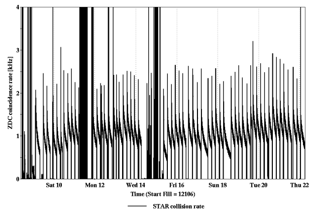
Figure 1: Luminosity monitoring using the ZDC coincidence rate for the full 19.5 GeV operation.
