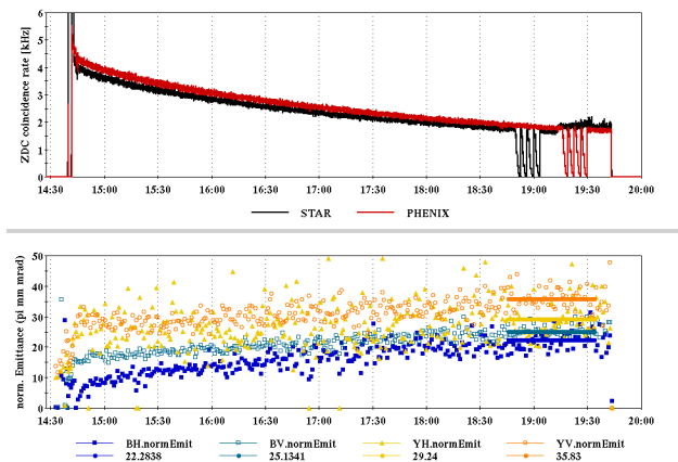
Figure 2: Store 12081 during the 31.2 GeV run with two vernier scans at the end. ZDC coincidence rate (top) and IPM emittance measurements (bottom).
