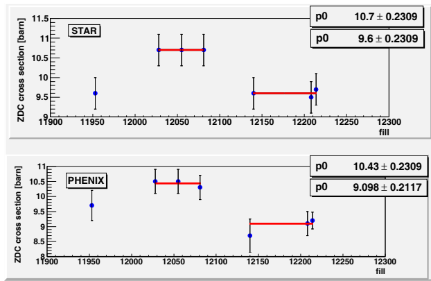
Figure 3: Effective ZDC cross sections during the two medium energy runs for the two experiments in FY10.
