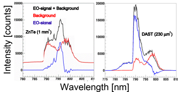
Figure 3: First BCD measurements with 230- \mu\text{m} thick organic DAST crystal compared with EO signals with a 1-mm inorganic ZnTe crystal. The both of the crystals were set 2.0 mm from the electron beam axis.
