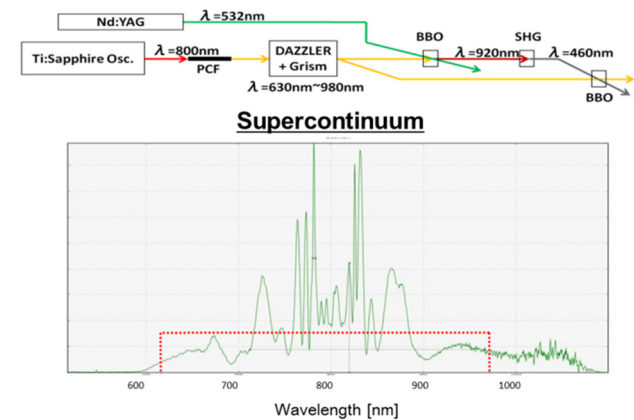
Figure 4: Schematic drawing of generation of broadband linear-chirped laser pulse with square-shaped spectrum (shaping region is shown as red dashed lines on supercontinuum spectrum). Pump source with 460 nm is not available commercially. It is generated from Nd:YAG laser (SHG: 532 nm) pump pulse and the supercontinuum signal pulse with additional NOPA stage.
