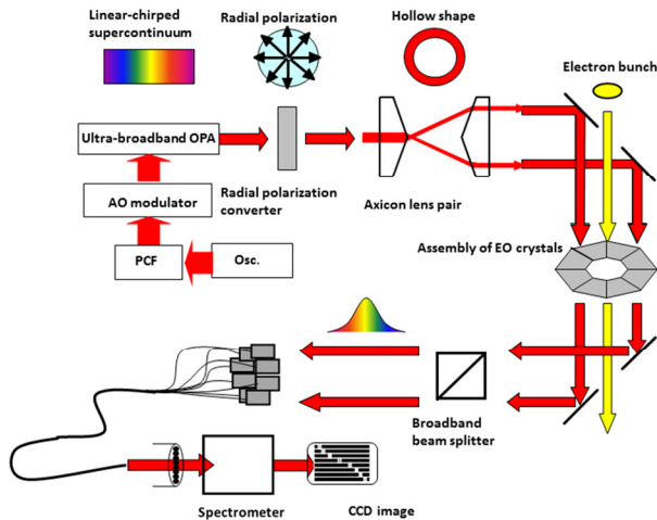
Figure 2: Schematic drawing of 3D-BCD monitor based on EO-multiplexing technique, utilizing simultaneous detection in imaging spectrographs with multi-track (eight tracks) of area array CCD of an image intensified (I.I.) camera.
