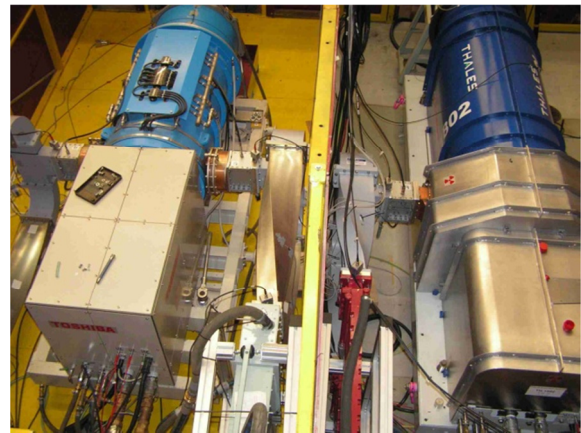
Figure 1: MBK test stands in DESY Hamburg
