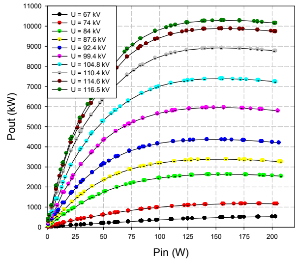
Figure 5: Gain curve for the different value of high voltage.
