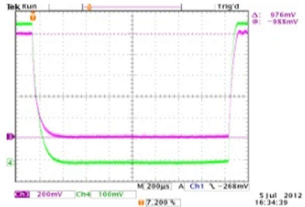
Figure 6: Wave shape of beam voltage and cathode current, the measurement from voltage and current monitors located inside CM.
