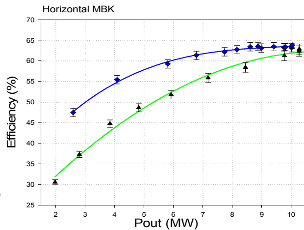
Figure 4: Efficiency for two types of MBK prototypes.
