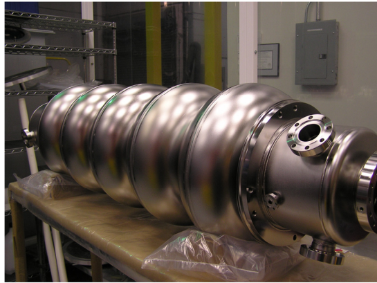
Figure 3: Niobium five-cell 704 MHz SRF cavity.
