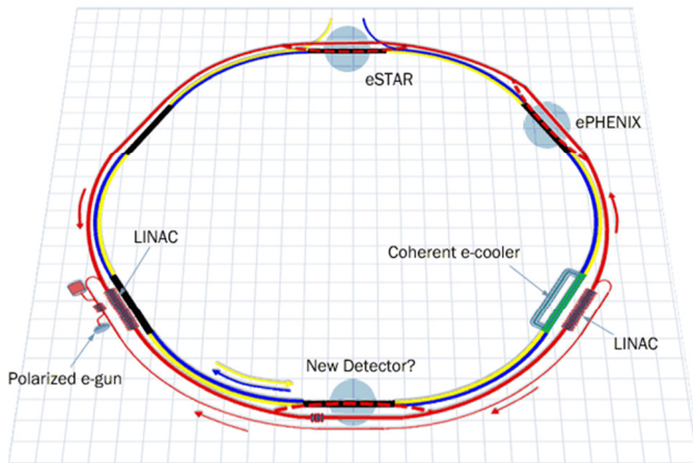
Figure 1: A schematic of the design for adding an electron ring (red), and possible future detector, to RHIC to create eRHIC, which would be the world's first electron-ion collider (EIC).
