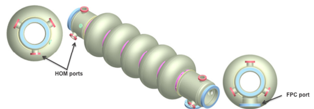
Figure 2: Schematic high-current 704 MHz SRF cavity.
