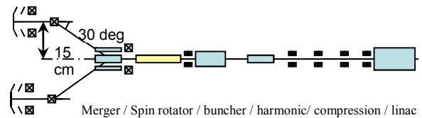
Figure 7: Schematic of the Gatling Gun injector.
