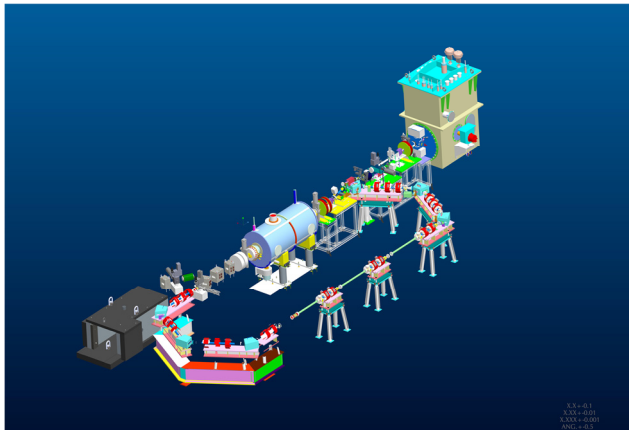
Figure 4: Schematic layout of the R&D Energy Recovery Linac at BNL. The electron gun is on the upper right side; the 5-cell accelerating cavity in the middle and the beam dump is on lower left.
