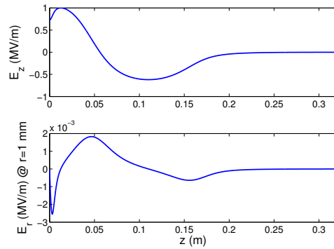
Figure 4: Field distribution ( E_z, E_r ) of a 1.4 cell gun cavity design with 35 mm exit iris and 53 mm beam tube radius.
