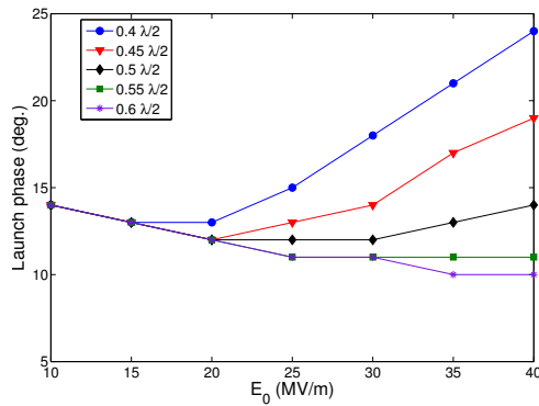
Figure 2: Energy-phase-field scan vs. half-cell length showing the phase with the highest energy gain in the half-cell.
