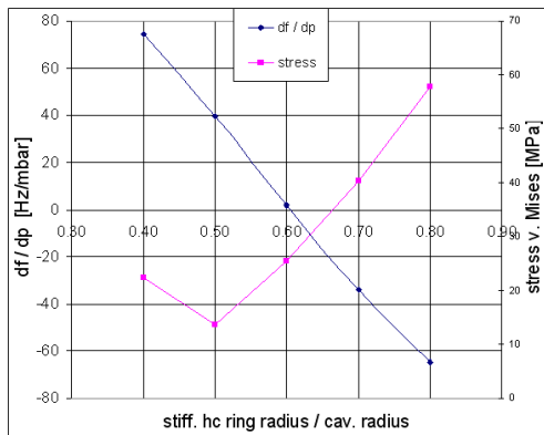
Figure 6: Detuning vs. LHe pressure coefficient and v. Mises stress versus position of a stiffening ring for the 1.4 cell design.
