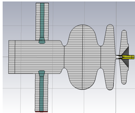
Figure 5: Possible design of the next 1.4 cell gun cavity featuring the HZDR-style choke cell, a modified cathode, two TTF-III type FPC having a 35 mm exit iris.
