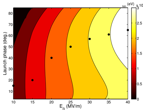
Figure 3: Energy-phase-field scan of a 1.4 cell cavity. The black dots denote the phase with the maximum energy gain at the given maximum on-axis field E_0 .
