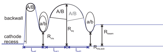
Figure 1: Geometry design parameters used for the cavity optimization scheme.
