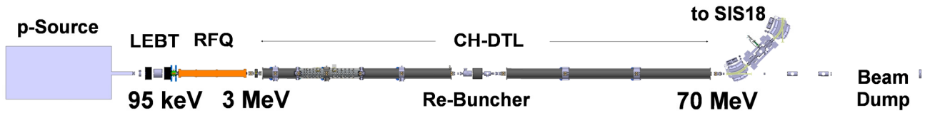
Figure 3: Layout of the FAIR proton linac.
