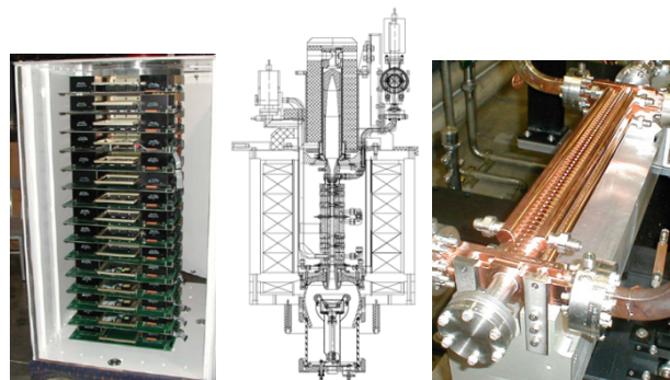
Figure 4: Solid state 400 kV modulator, SLAC XL4 50 MW 1.5 \mu\text{s} X-band klystron, and a T53 X-band accelerator structure.
