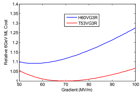
Figure 6: Dependence of the X-band 6 GeV main linac cost on acceleration gradient for the two structure types, normalized to the minimum for T53.
