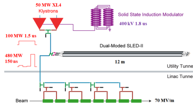
Figure 3: X-band rf unit layout. A pair of 50 MW klystrons sharing a modulator and an rf pulse compressor, powers several (6–9) traveling-wave accelerator structures.
