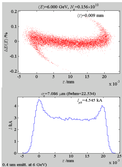
Figure 2: Litrack simulation results for longitudinal phase space and current profile after Linac-3 showing ~3 kA peak current in the bunch core and almost no energy-z correlation (bunch head is at z < 0 ).
