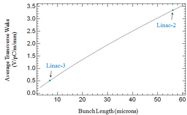
Figure 5: Transverse wakefield in the H60 structure averaged along the length of the bunch as a function of bunch length. The values for the design bunch lengths before and after the second bunch compressor are indicated.
