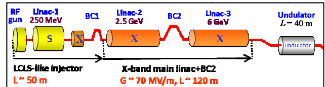
Figure 1: Schematic layout of a compact X-ray FEL driven by the X-band linear accelerator.
