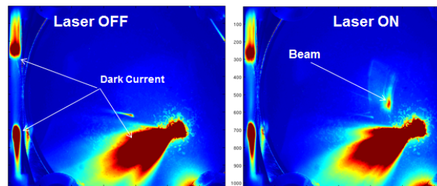
Figure 6: First evidence of photoemitted beam on a dummy cathode.
