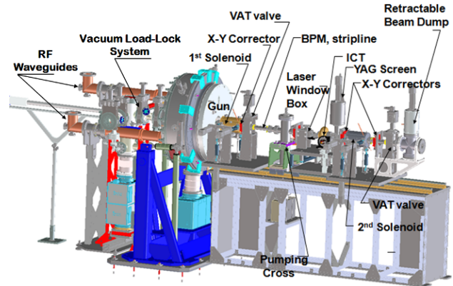
Figure 2: APEX Phase 0 layout.
