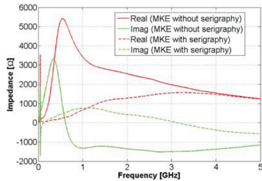
Figure 4: CST simulations of the longitudinal impedance for the SPS extraction kicker (MKE-L) with and without serigraphy.
