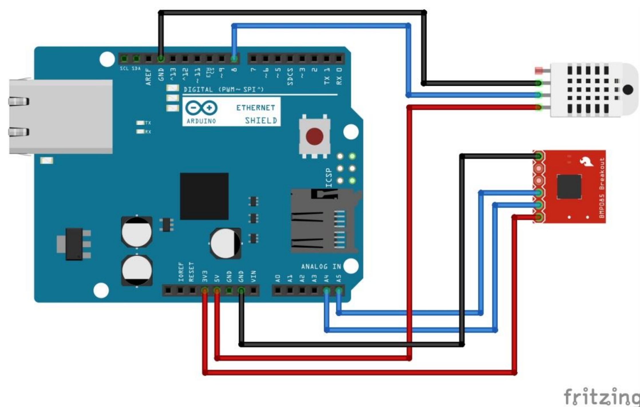
Figure 1: Circuit Diagram
