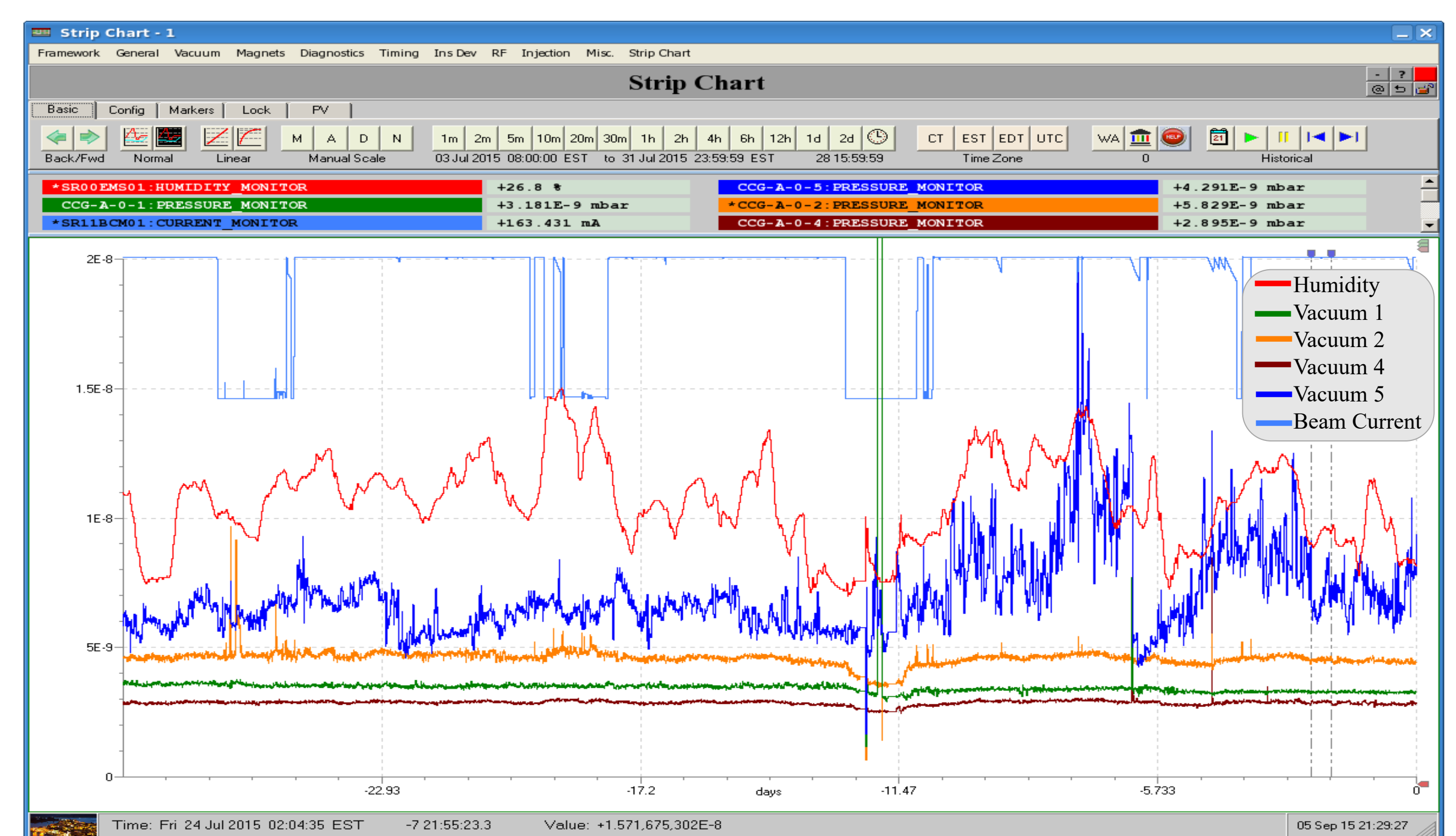
Figure 3: Humidity and LINAC Vacuum vs Time
