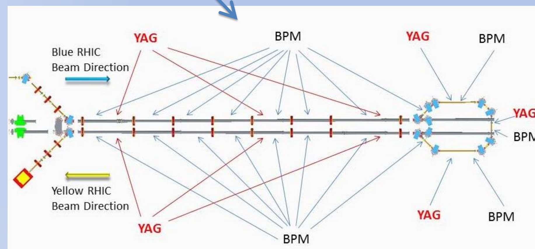
Figure 4: Electron beam diagnostics in the cooling and U-turn region, YAG is a screen transverse profile monitor.
