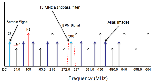
Figure 7: Using a 109MHz clock places the 300MHz signal in the first Nyquist zone.
