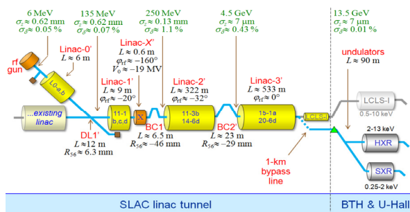
Figure 1: LCLS-II structure layout [2].
