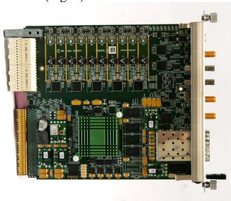
Figure 6: Struck SIS8300 digitizer.
