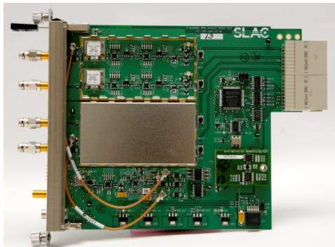
Figure 2: SLAC built BPM analog front end.
