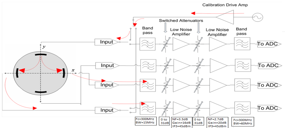
Figure 5: BPM calibration process.
