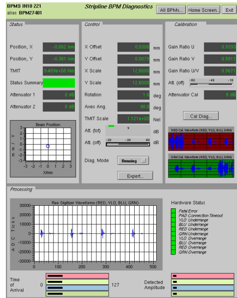
Figure 8: EPICS EDM user interface.
