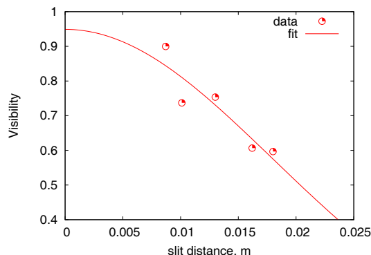
Figure 6: Horizontal visibility as a function of slit separation.
