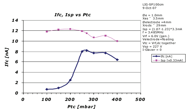
Figure 2: Faraday Cup current (Ifc) vs. the pressure in the gas cell (Ptc).
