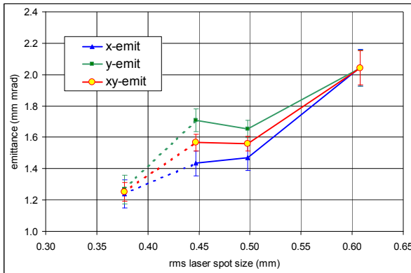
Figure 2: Measured normalized projected emittance as a function of the rms laser spot size at the cathode for a bunch charge of 2 nC. The geometric mean xy-emittance is defined as \epsilon_{xy} = \sqrt{\epsilon_x \epsilon_y} .
