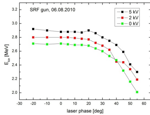
Figure 5: Measurement of the kinetic electron energy as function of laser phase for an acceleration gradient of 6 \text{ MV/m} ( 16 \text{ MV/m} peak field) and different DC voltages at photo cathode.
