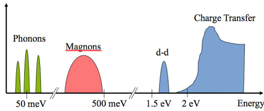
Figure 2: Typical excitation spectrum of a solid state system.
