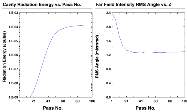
Figure 3: Intracavity pulse energy (left) for a sample 14-keV XFEL-O example and the time-integrated far field angle (right) of the intracavity radiation as a function of pass number.
