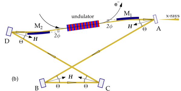
Figure 1: XFEL-O configuration with four Bragg crystal reflections on the return path.
