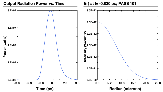
Figure 4: Temporal and radial power profile for pass 101 as measured in the center of the undulator.
