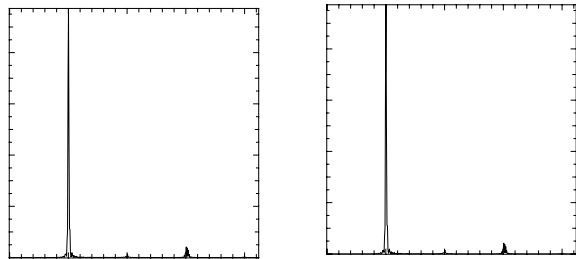
Figure 3: On-axis, far field spectrum |E(\omega)| from a pre-bunched beam propagating in (left plot) a "normal", single frequency undulator with a_{u,1} = 1.0 and (right plot) a in biharmonic undulator with \lambda_{u,2} = 3\lambda_{u,1} , a_{u,1} = 1.0 and a_{u,2} = 1.5 .
