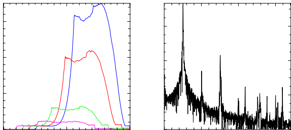
Figure 2: Boosted frame simulation results for a FEL amplifier seeded with 10 MW of input power at 200-nm wavelength. The left plot shows increasing P(t) traces at z = [0.5, 0.7, 0.9, 1.0] m. The right plot shows the on-axis, far field spectrum (a.u.) for z = 1.0 m.
