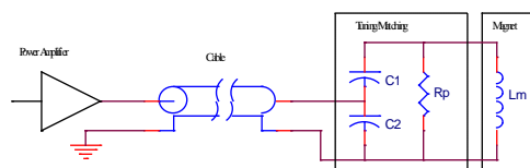
Figure 2: RHIC AC-dipole simplified schematic.
