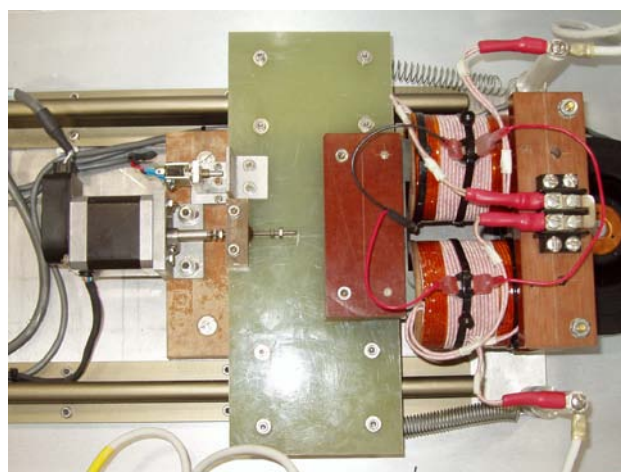
Figure 6: Tuning coil assembly
