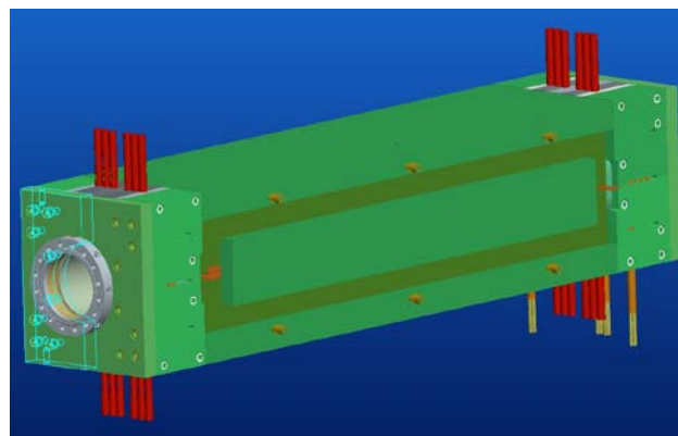
Figure 5: RHIC Spin Flipper high-Q AC-dipole 3D view
