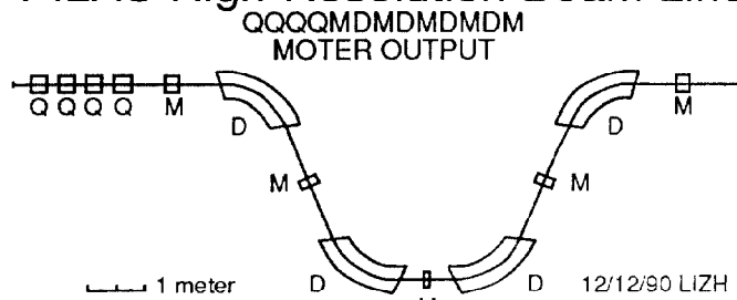
Figure 4. High resolution beam line for PILAC.
