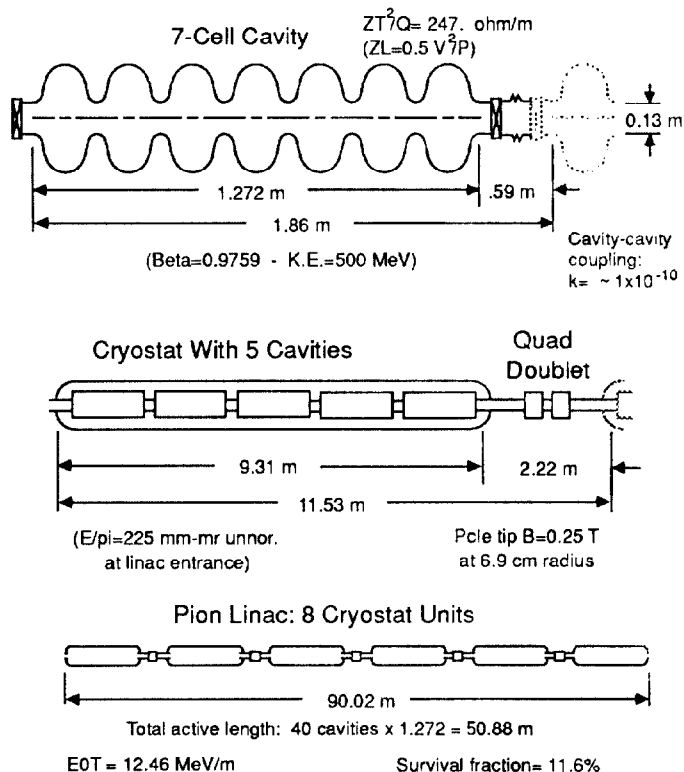
Figure 3. Reference design of pion linac.
