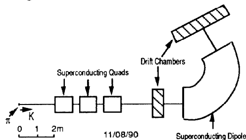
Figure 5. High-resolution spectrometer for PILAC.
