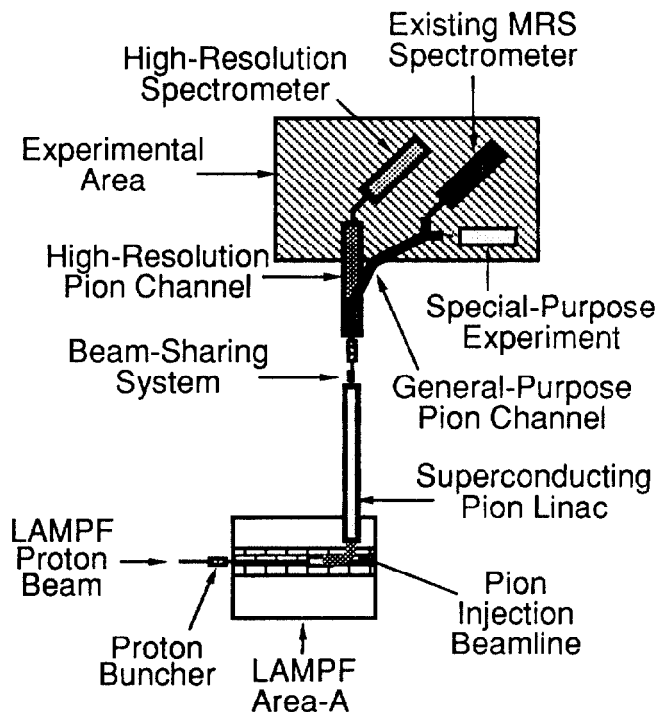
Figure 1. Concept for PILAC facility at LAMPF.
