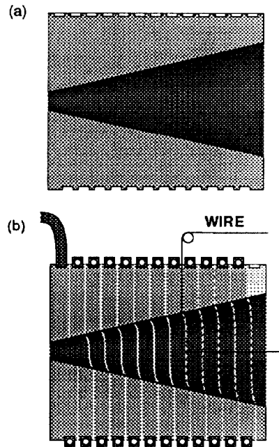
Figure 2. FC body cross section: (a) Showing internal cone and grooves from rectangular conductor; (b) Showing EDM
