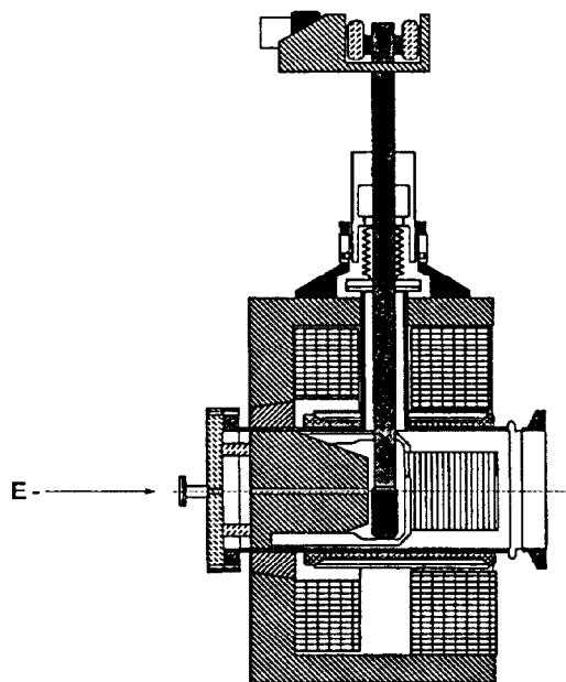
Figure 3. Complete target module assembly showing trolley target driven from above, TFS surrounding both the target (solid black) and FC, and the FC itself supported by the TFS yoke (hashed) on the upstream end.
