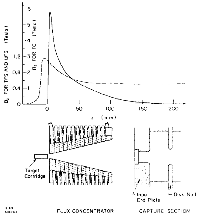
Figure 1. The positron source adiabatic system. The devices shown in cross section at bottom are to scale. The computed solenoidal fields and measured FC pulsed field are shown above with the same z -scale as for the devices.
