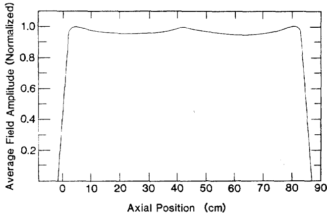
Fig. 2 Longitudinal field variations measured by bead pull perturbation techniques.
