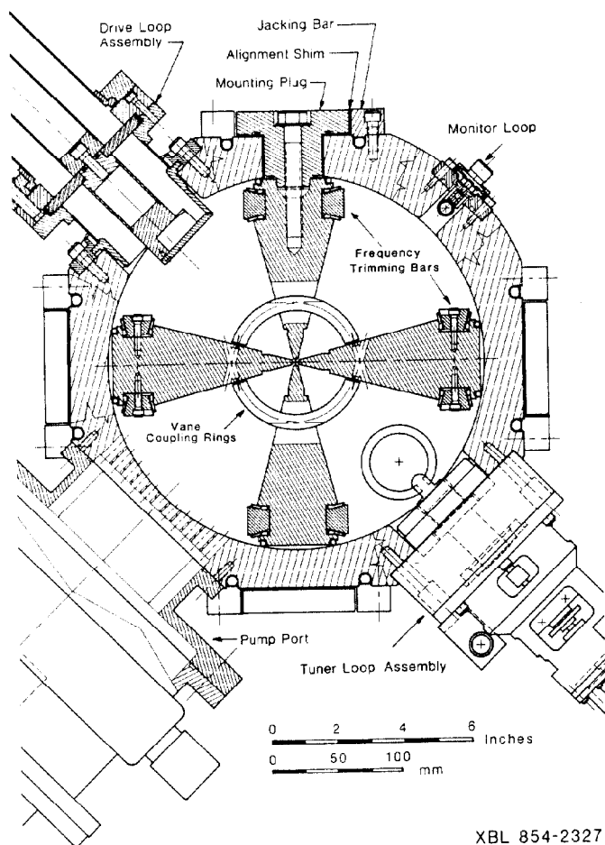
Fig. 1 Composite cross sectional view of the RFQ.
