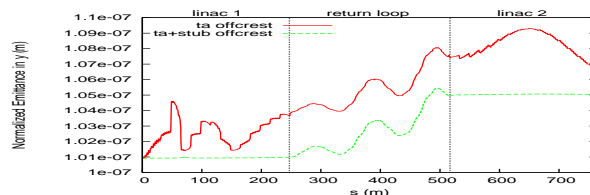
Figure 3: Emittance growth with off crest operation with and without symmetrizing stub.
