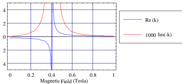
Figure 6 Variations of the off diagonal elements of the relative magnetic permeability tensor, k , with magnetic field.
